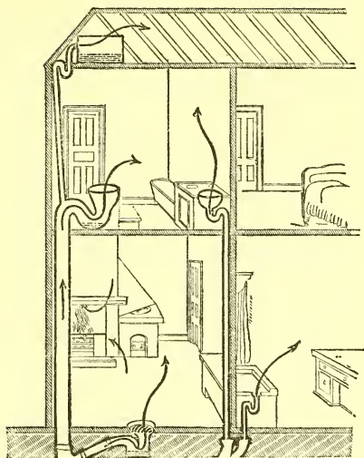
FIG. 30.—Unused traps, with water evaporated.
